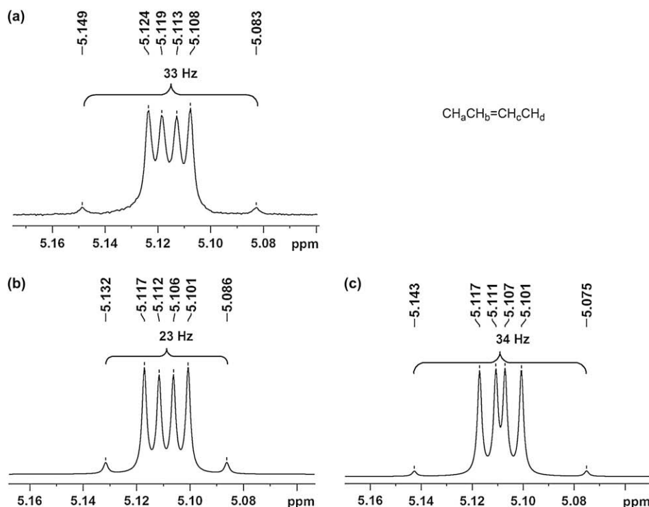
Figure 1. Comparison of the ^1\text{H} NMR (500 MHz) resonance for the olefinic proton on dimer 11 : (a) experimental resonance at \delta_{\text{Hb}}=5.11 ppm, (b) simulated resonance for the Z -isomer: \delta_{\text{Hb}}=5.109 ppm, coupling constants (Hz) J_{\text{ab}}=8 ; J_{\text{ac}}=0.2 ; J_{\text{bc}}=10 ; J_{\text{ad}}=0 , (c) simulated resonance for the E -isomer: \delta_{\text{Hb}}=5.109 ppm, coupling constants (Hz) J_{\text{ab}}=8 ; J_{\text{ac}}=0.2 ; J_{\text{bc}}=16 ; J_{\text{ad}}=0 (simulations with NMR-SIM TOPSPIN 2.1).
